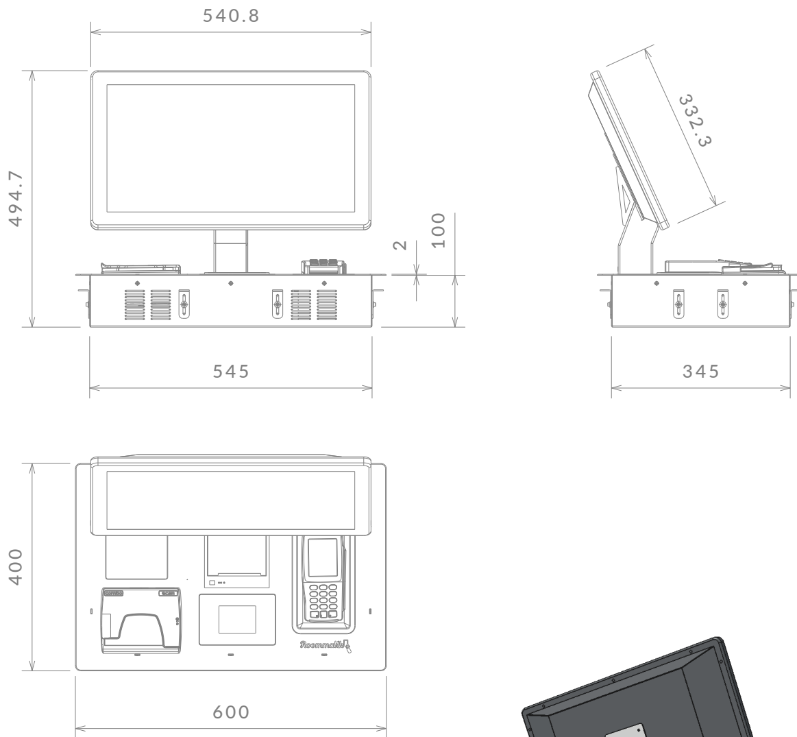
KIOSK S-600 main dimensions
